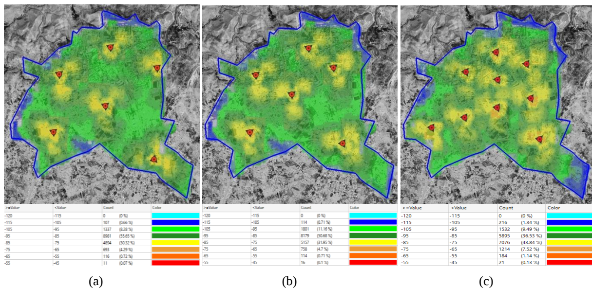
Figure 4: Coverage by Signal Level According to PGM model for (a) Layout 1 (b) Layout 2 (c) Layout 3
