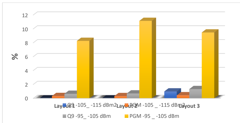
Figure 6: Error Rate Comparison Across Layouts and Signal Conditions for PGM and Q9 Models
